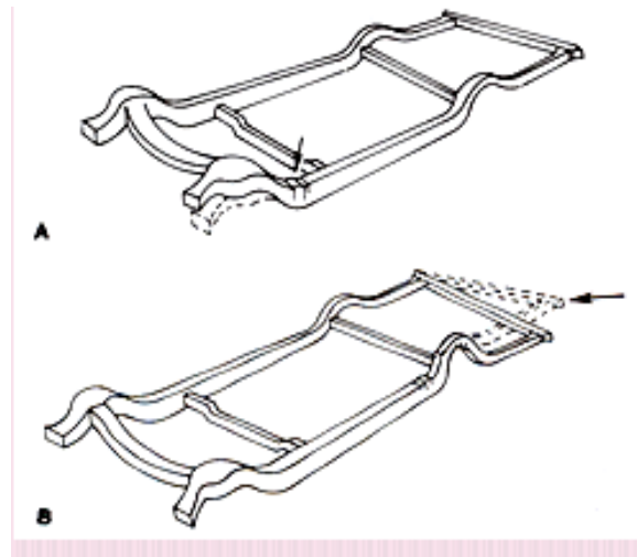
Fig. 9: (A) Note the sag condition on the left front frame section and (B) rear end sag.
